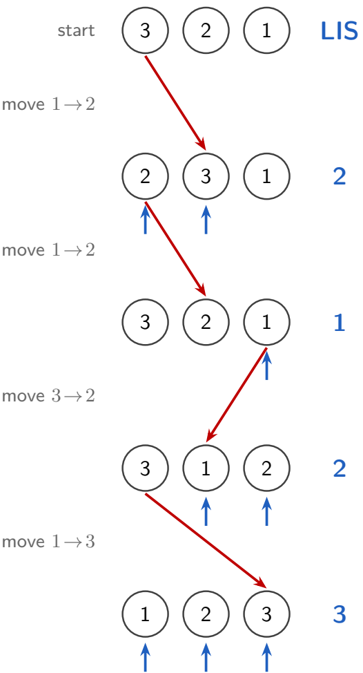
Figure H.1: Visualization of the interaction in the second example. At the start all the historic events are in reverse order. The red arrows show the operations, and the blue arrows show a possible Longest Increasing Subsequence (it may not be unique).
