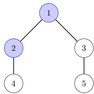
Figure G.1: An optimal solution for the second sample. Brother Duck can install CCTV cameras at the blue vertices 1 and 2, with which he can uniquely determine the hideout of the gang. It can be proven that Brother Duck needs at least 2 cameras.
