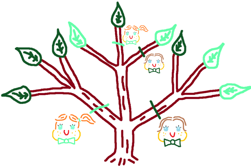
Figure A.1: An example of a tree of height 2, like in Sample Input 4. In this instance of a tree, the final leaf is teal.
